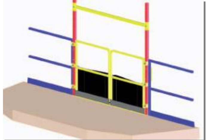
The Self-Closing Pallet Gate in the closed position offers full-height edge of mezzanine protection with its 42" top-rail, mid-rail, and adjustable 4" toeboard.
